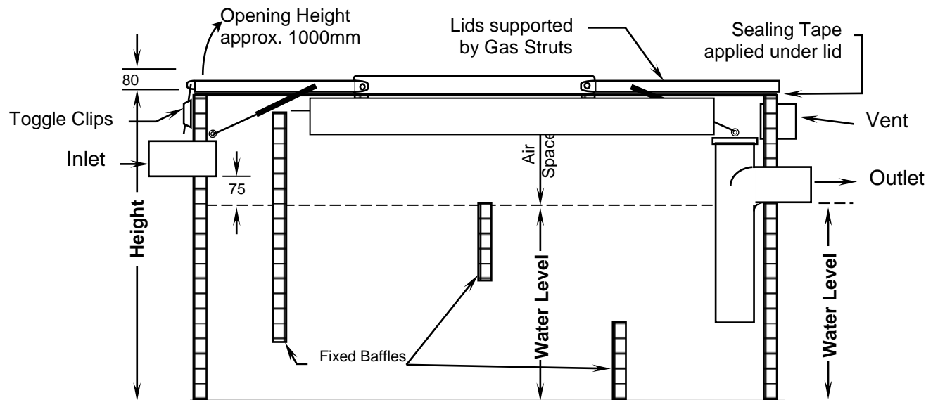
SECTION X-X
