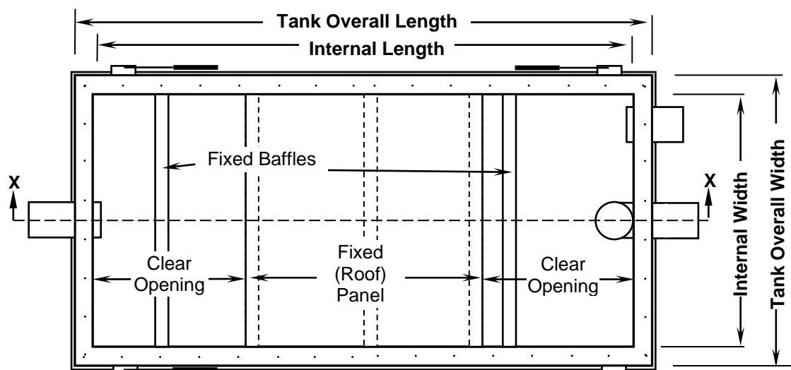
PLAN VIEW
