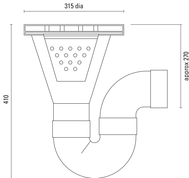
Section View Silt Trap Assembly
