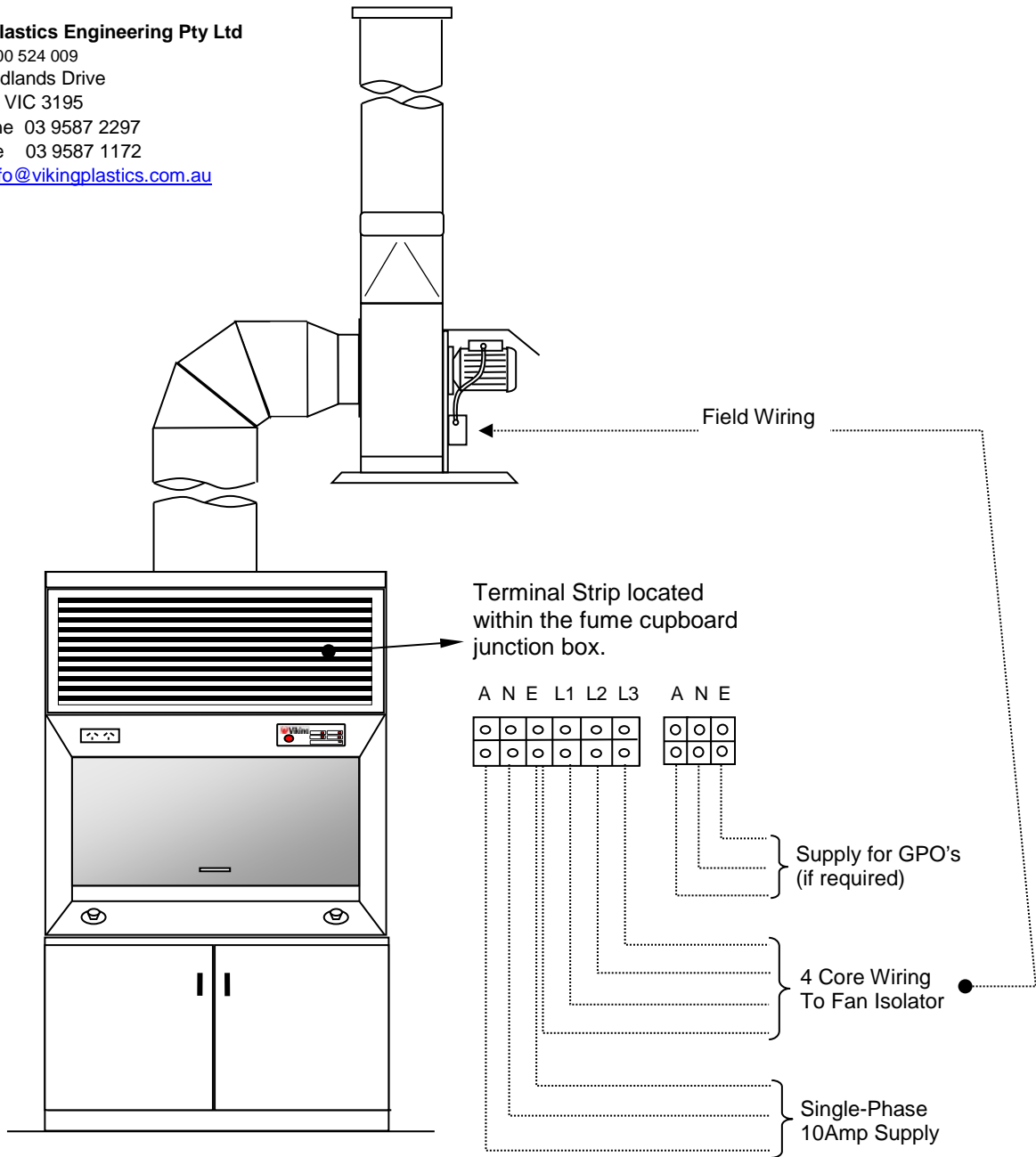
Wiring Diagram
